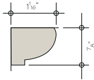
Cove Moulding
