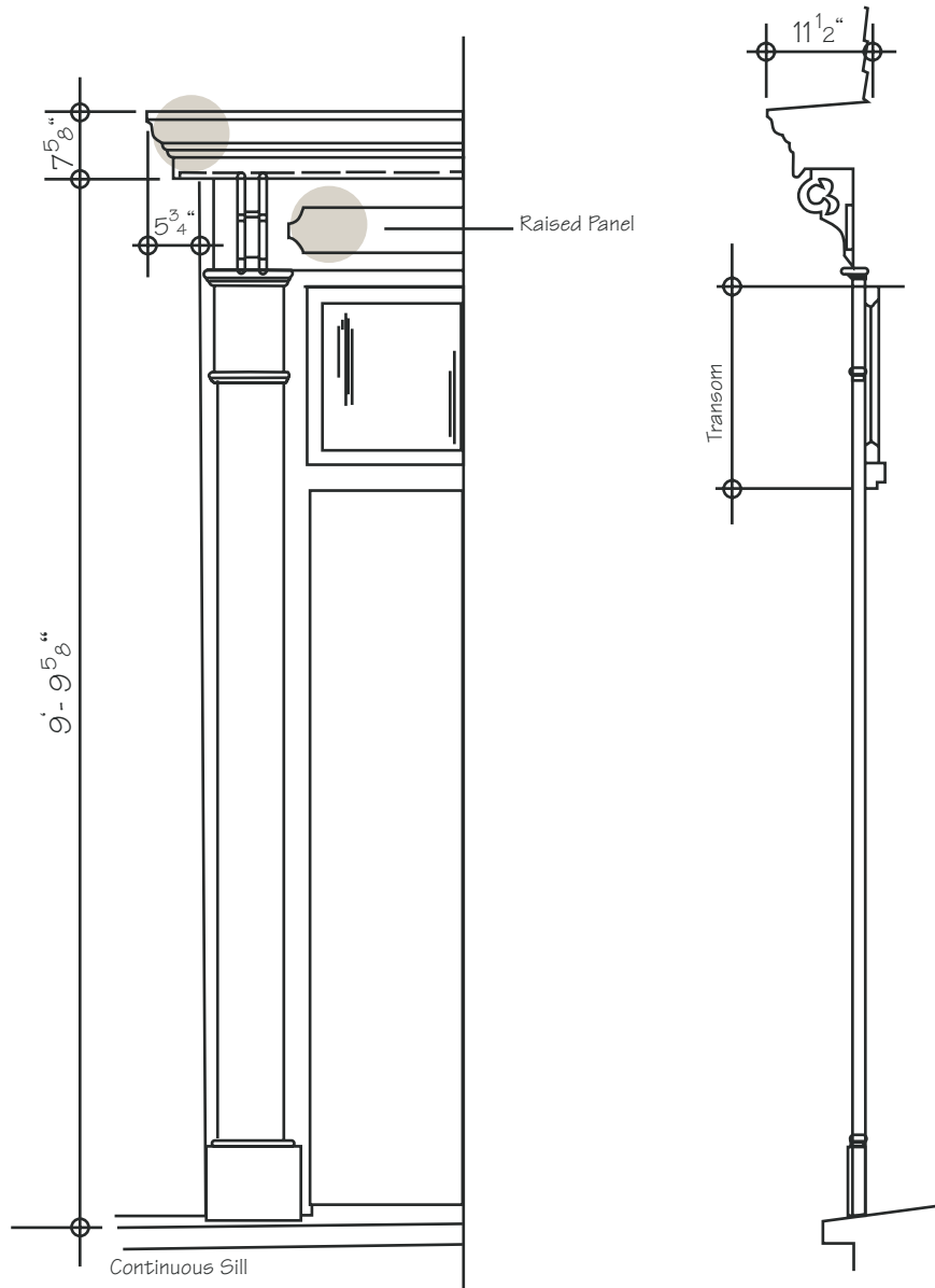
1/2 ELEVATION
