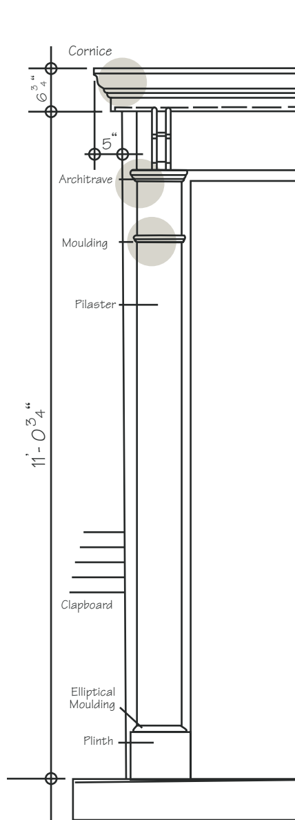
\frac{1}{2} ELEVATION
