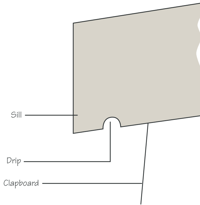
Sill Detail-2nd Floor
